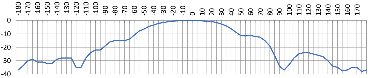
1800Mhz Yagi, vertical polarity
