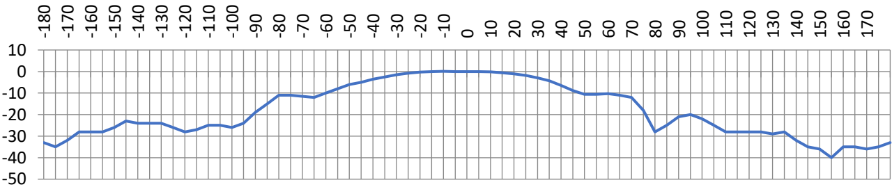
2100Mhz Yagi, vertical polarity
