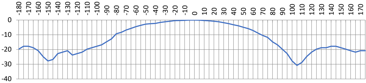
800Mhz Yagi, vertical polarity
