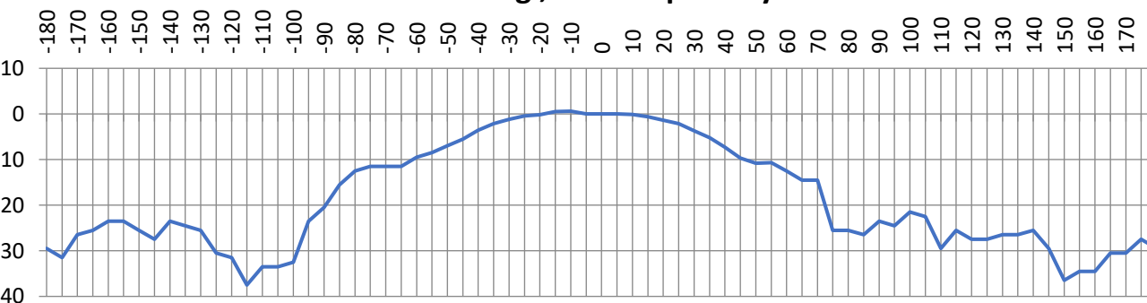
2600Mhz Yagi, vertical polarity
